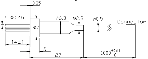
Vertical Flange
