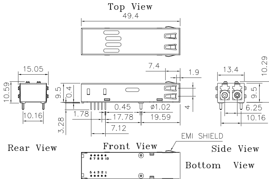
TRML-9100FEG / TRML-9100FAEG
